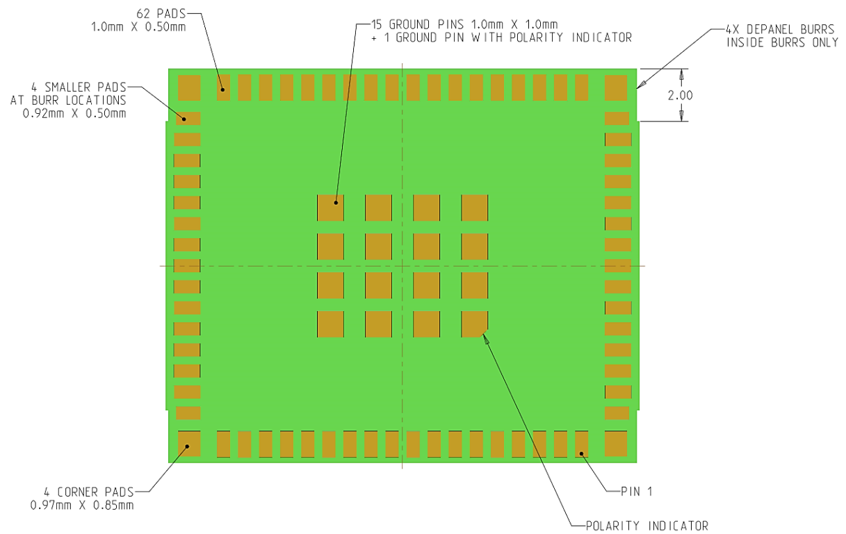
Figure 5-3: Footprint Drawing
