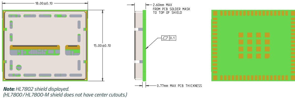
Figure 5-1: Mechanical Drawing
